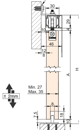
STANDARD A= H-43
