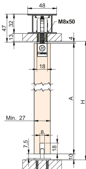
CONJUNTO | SET | JEU FUNDA | SUPPORT | COUVERTURE FT + STAR
